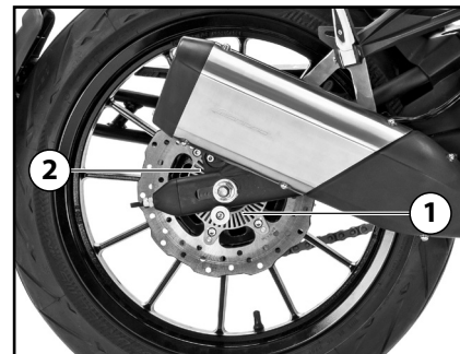
1. Rear sensor rotor 2. Rear wheel sensor
